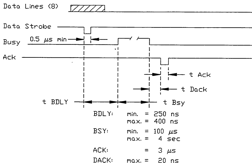
Figure 3.4 Parallel Data Timing (upwards Centronics Compatible)
